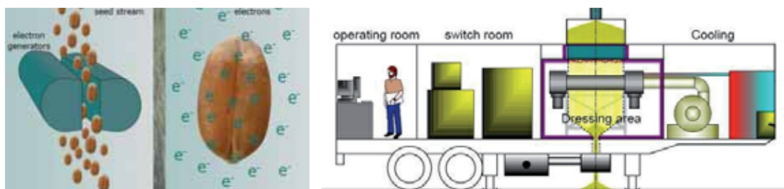
Fig. 13 Treatment of Seed with Electrons. Principle (left), Practice (right) (Source: Schmidt-Seeger)
