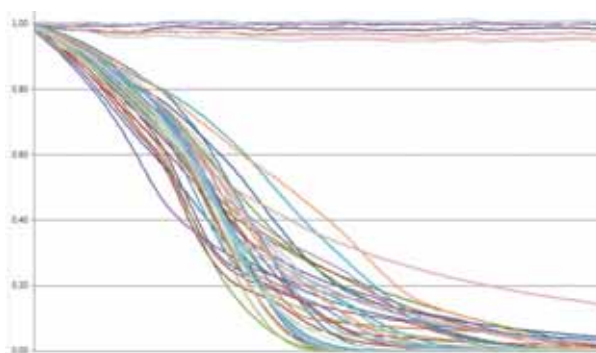
Fig. 5 Curves showing Oxygen Depletion of 96 Seeds (Source: Astec Global)
